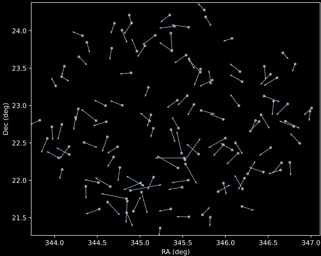
APOGEE DR17 Cluster 1 Proper Motion Vectors (n=121)
