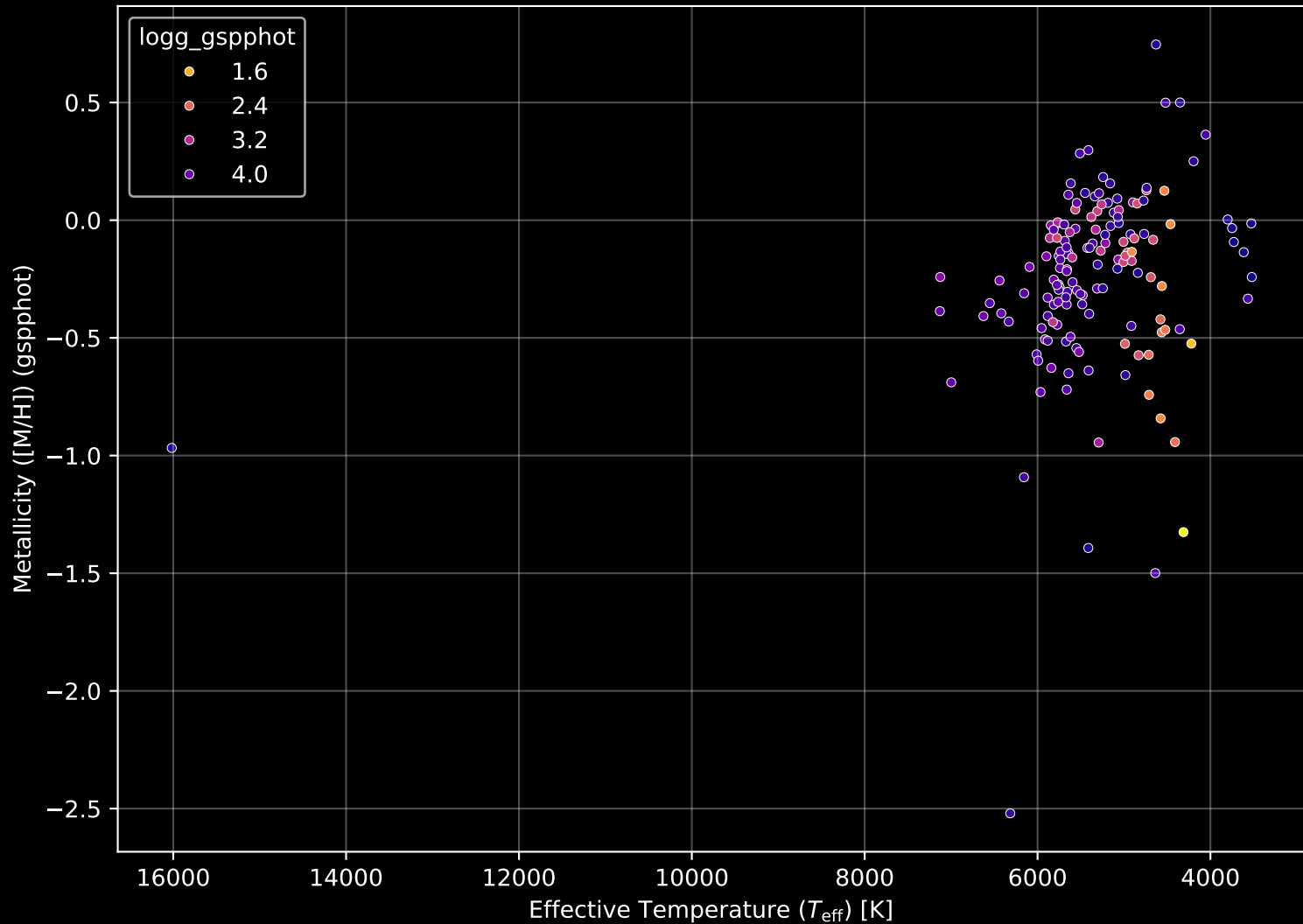
APOGEE DR17 Field: [040+43_MGA] Stellar Population Parameters (n= 152)
