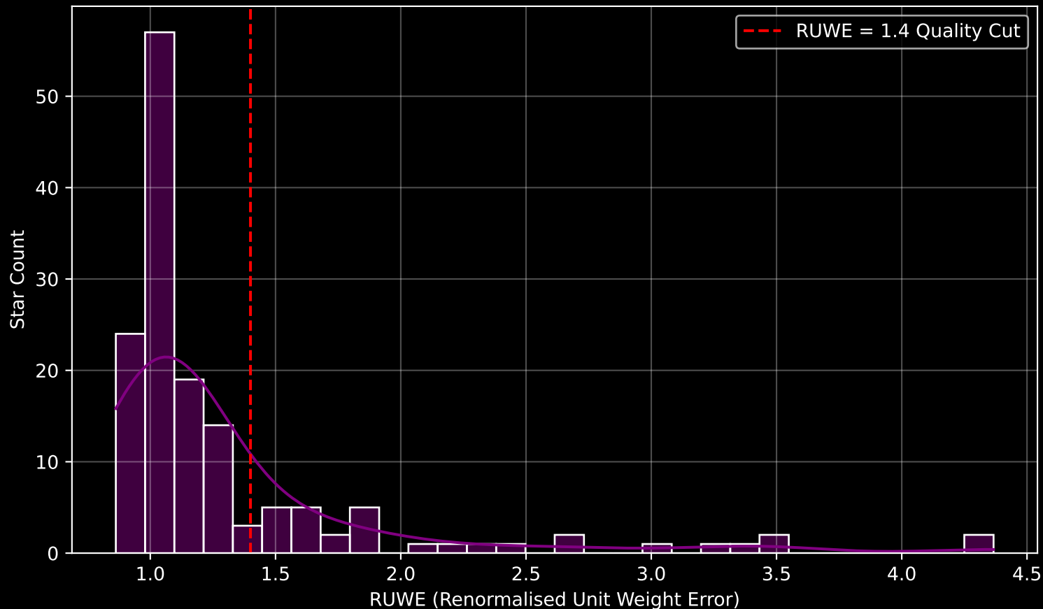
GAPOGEE DR17 Field [040+43_MGA] RUWE Distribution (n= 147)
