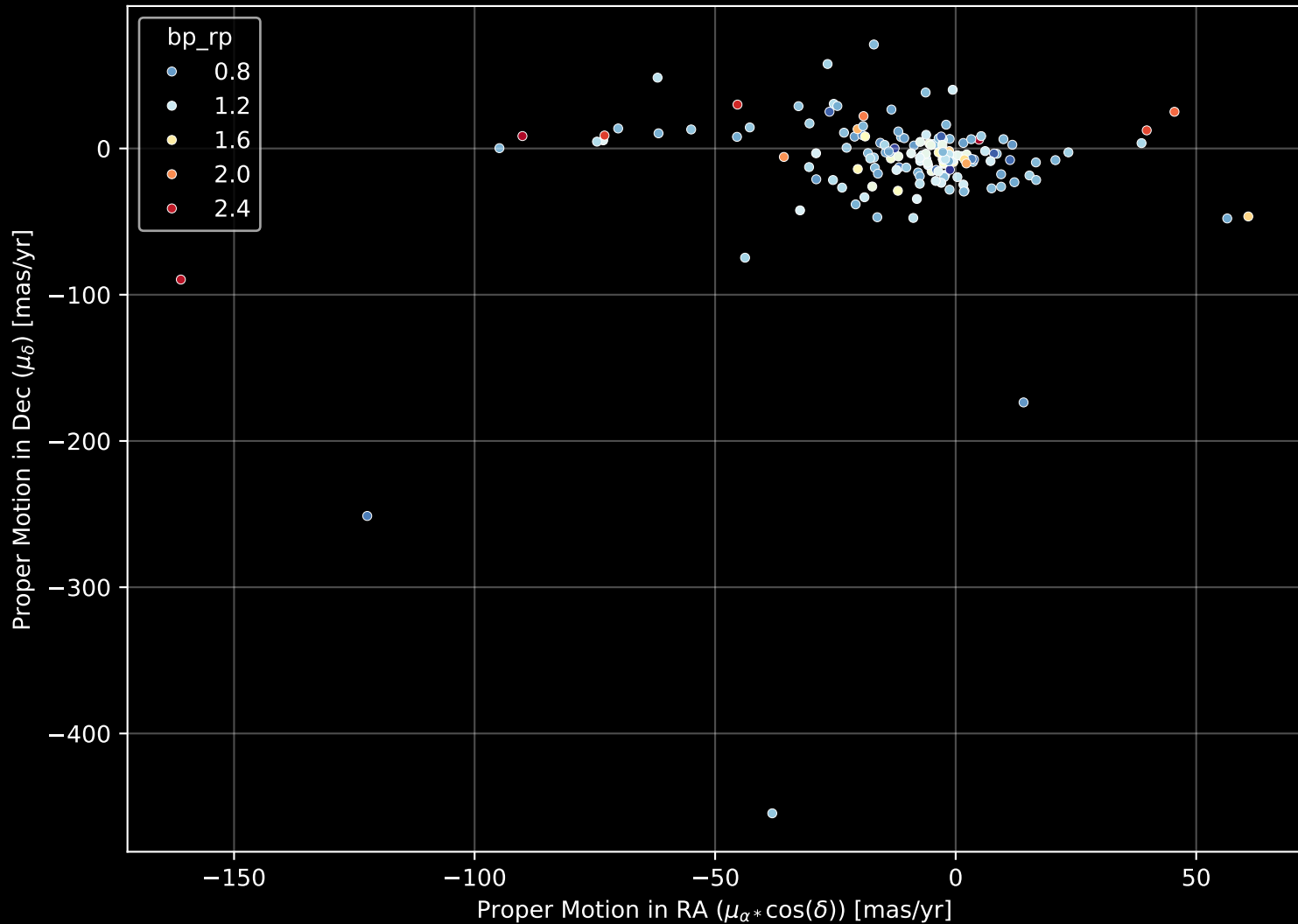
APOGEE DR17 Field: [040+43_MGA] Proper Motion Diagram (n= 152)
