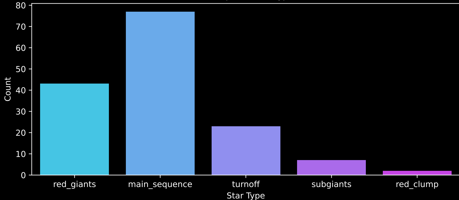
APOGEE DR17 Field: [040+43_MGA] Count plot of Star Type
