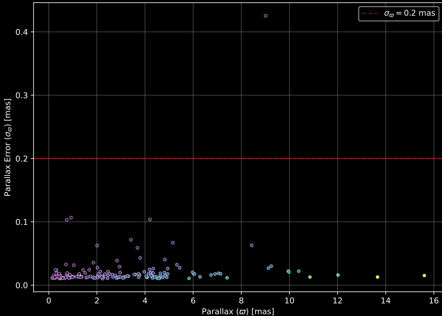
APOGEE DR17 Field: [040+43_MGA] Parallax Quality (n= 152)
